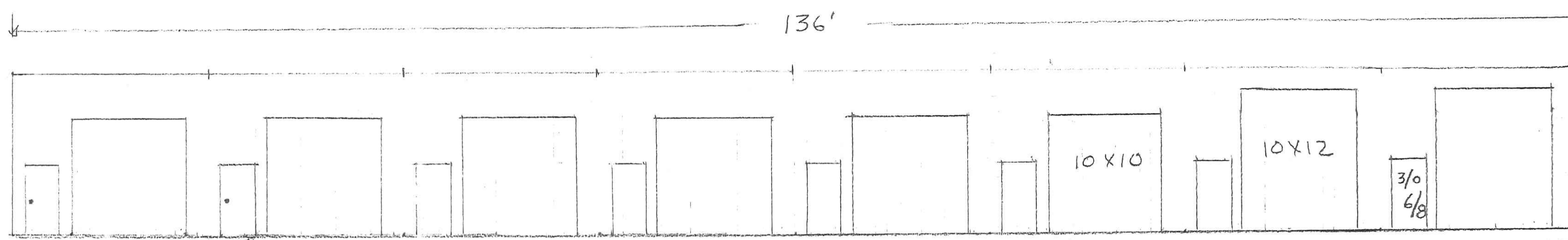
FRONT ELEV. 1/8" = 1'
